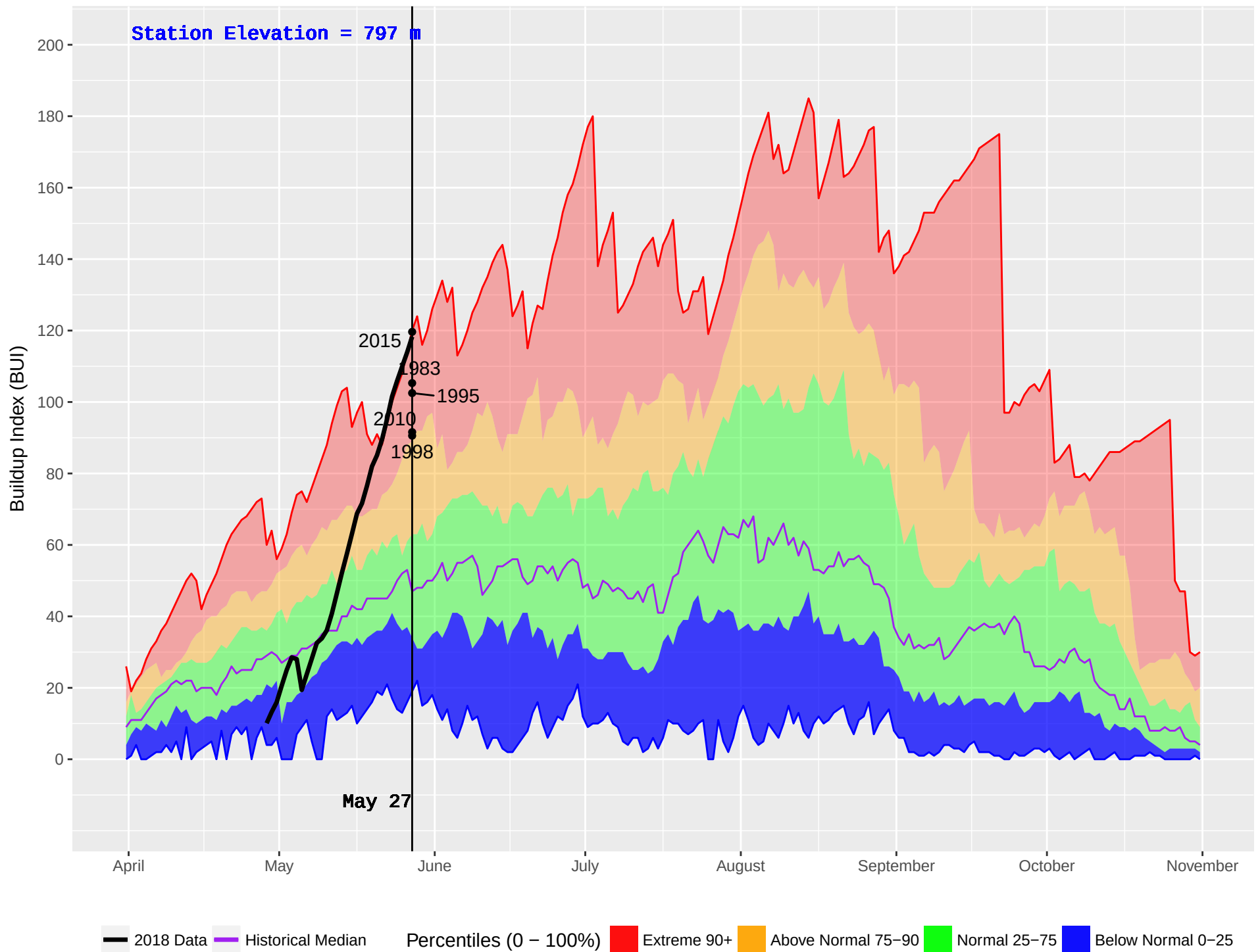
VALEMOUNT HUB (194) : Historical (1970–2016) and Current (2018) Noon Buildup Index (BUI)
