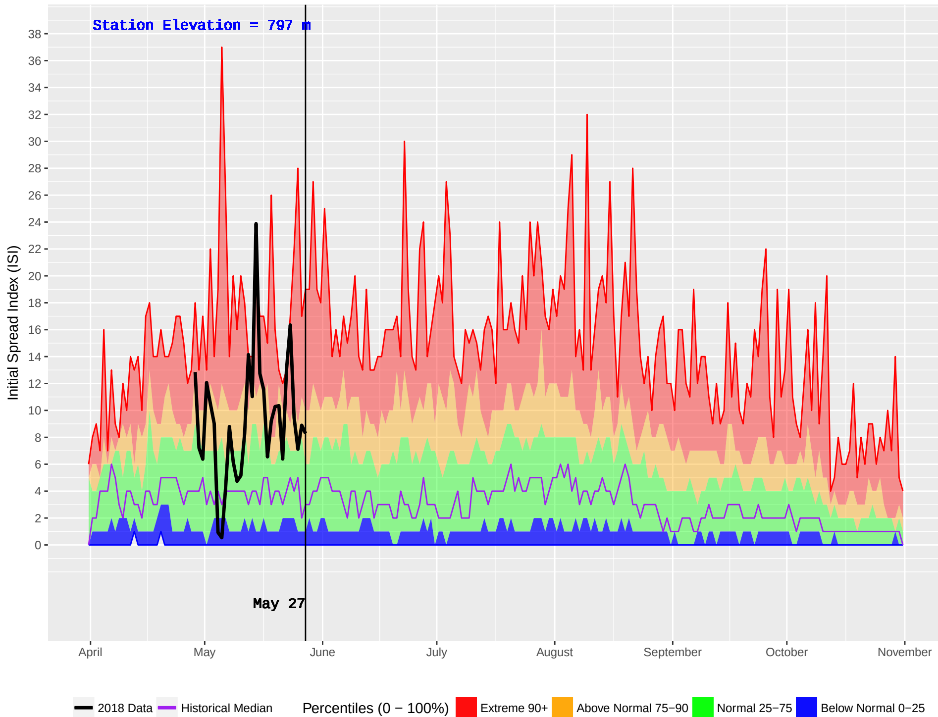
VALEMOUNT HUB (194) : Historical (1970–2016) and Current (2018) Noon Initial Spread Index (ISI)
